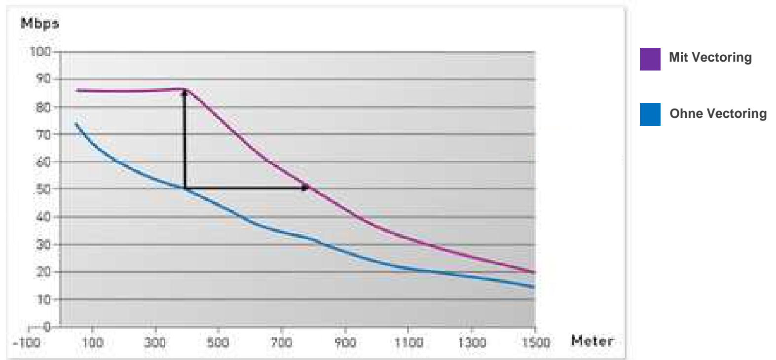
Figure 1: Vectoring-enhanced downstream bandwidth
